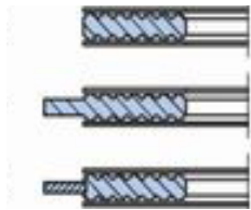
620 Basic Type Kammprofile Gasket
